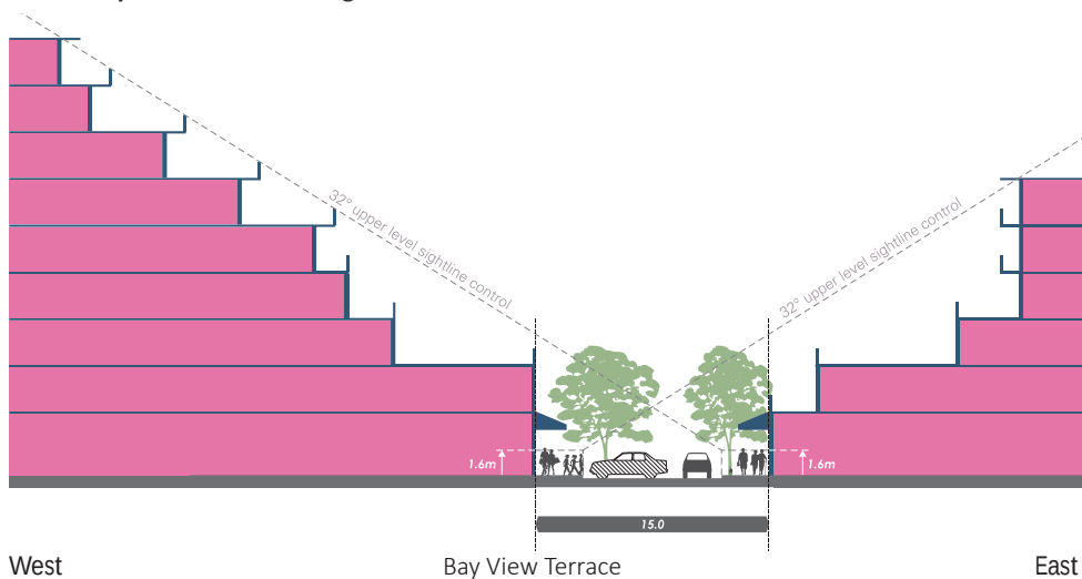
West East Figure 28: Section C - Bay View Terrace - north (15.0m) characterised by single storey heritage facade (east) with nil podium setbacks and upper level street setbacks determined by specified sight lines.
