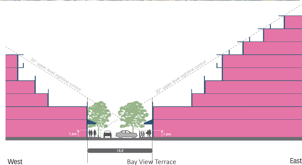
West East Figure 30: Section D - Bay View Terrace - south (15.0m) characterised by two storey heritage facades with nil podium setbacks and upper level street setbacks determined by sight lines from public realm.
