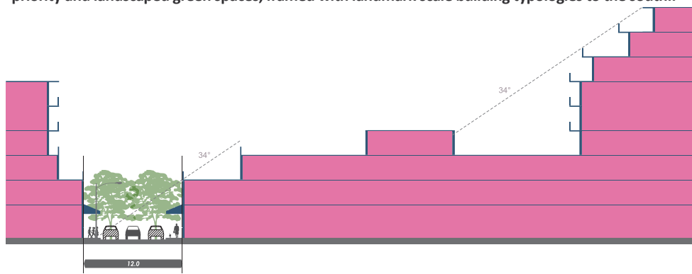
South North Figure 27: Section B - St Quentin Avenue (12.0m) characterised as a slow speed pedestrian space framed by human scale buildings and no street setbacks.
